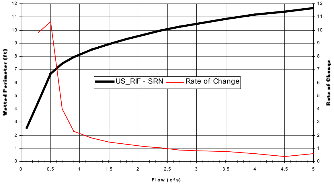
Crater Creek Above Diversion US_RIF - SRN Wetted Perimeter vs Flow
